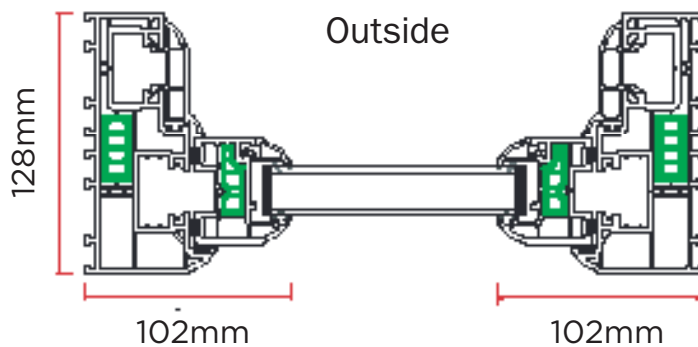
Horizontal Section Through Bottom Sash
