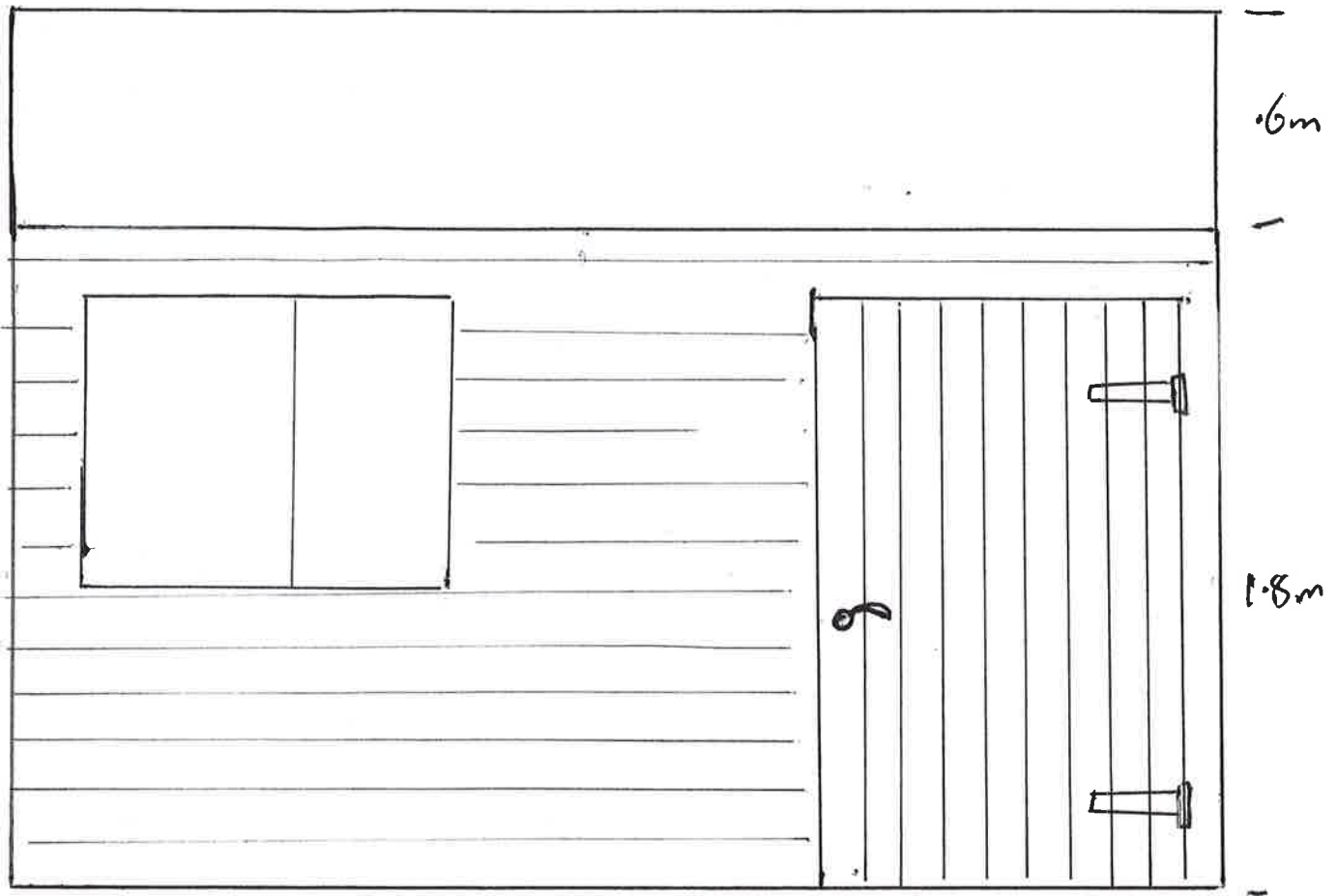
South Elevation 3.3m 150mm shiplap with Felt Roof
