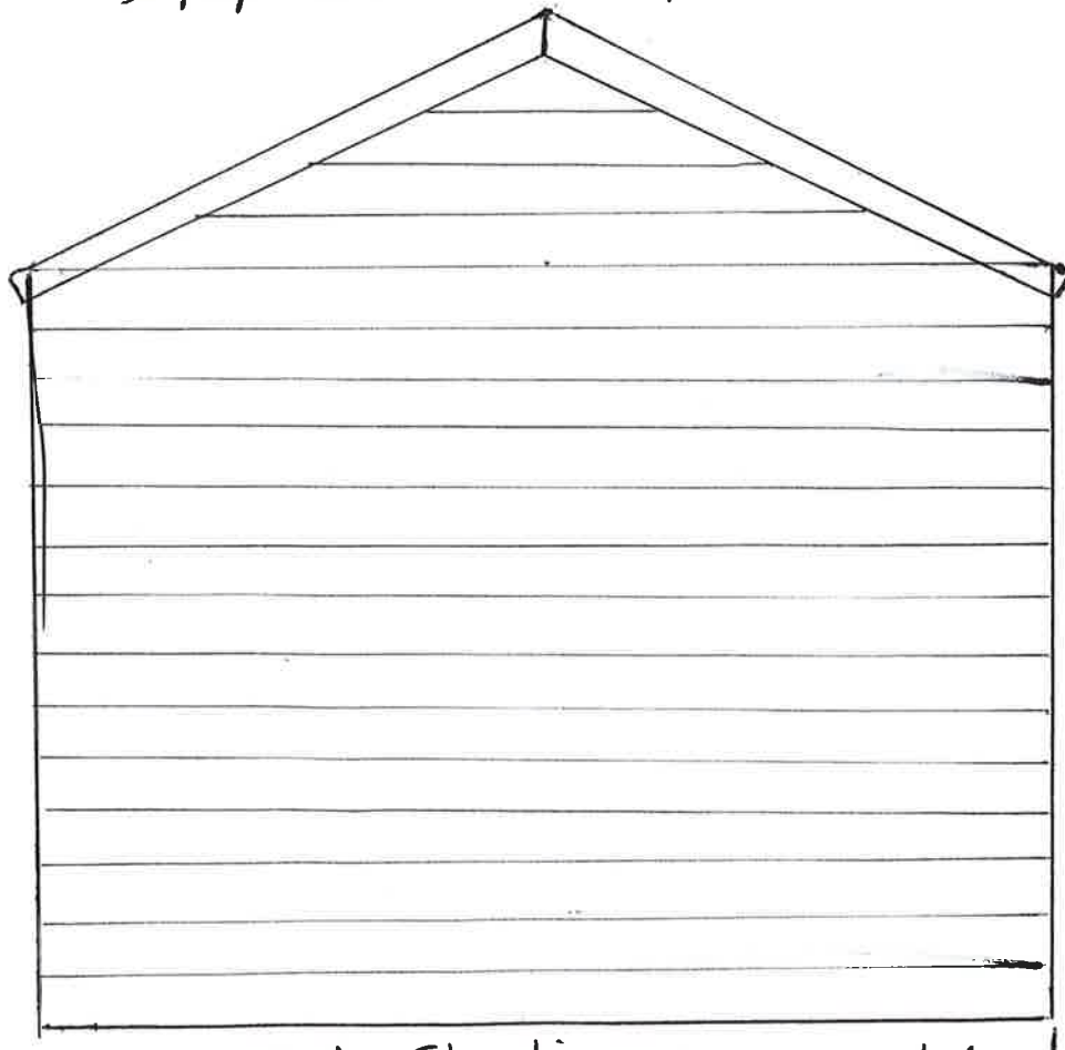
West & East Elevation 2.4m. Solid 150mm shiplap
