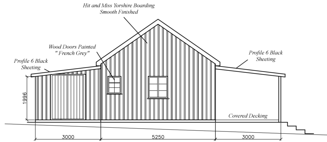
South West Elevation (Side)
