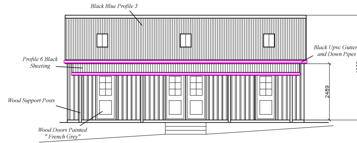
South East Elevation (Front)
