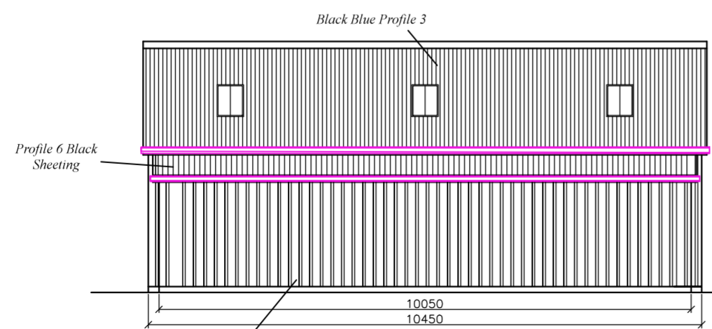
North West Elevation (Rear)
