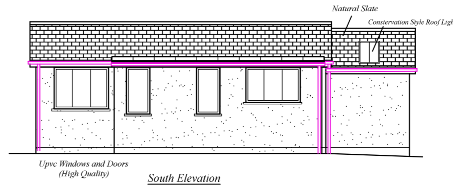
South Elevation
