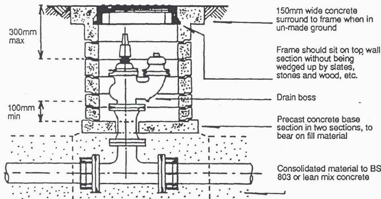
Drawing of pit chamber to BS 5306 : part 1 : 1976 (1983)
