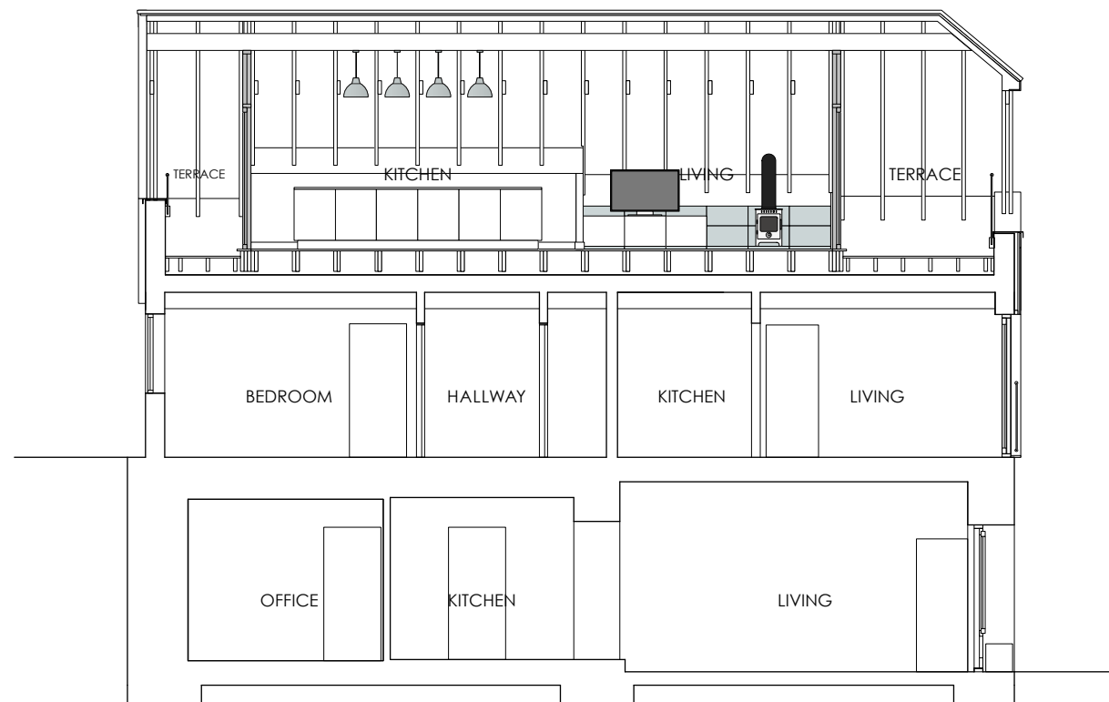
SECTION B-B
