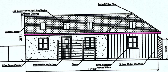
Proposed West Elevation
