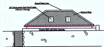
Proposed South ( Road Side) Elevation
