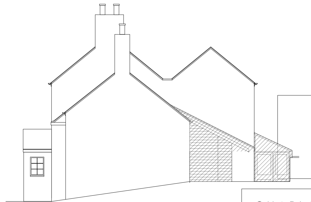
NORTH ELEVATION
