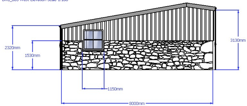
DRG_005 West Elevation Scale 1:100
