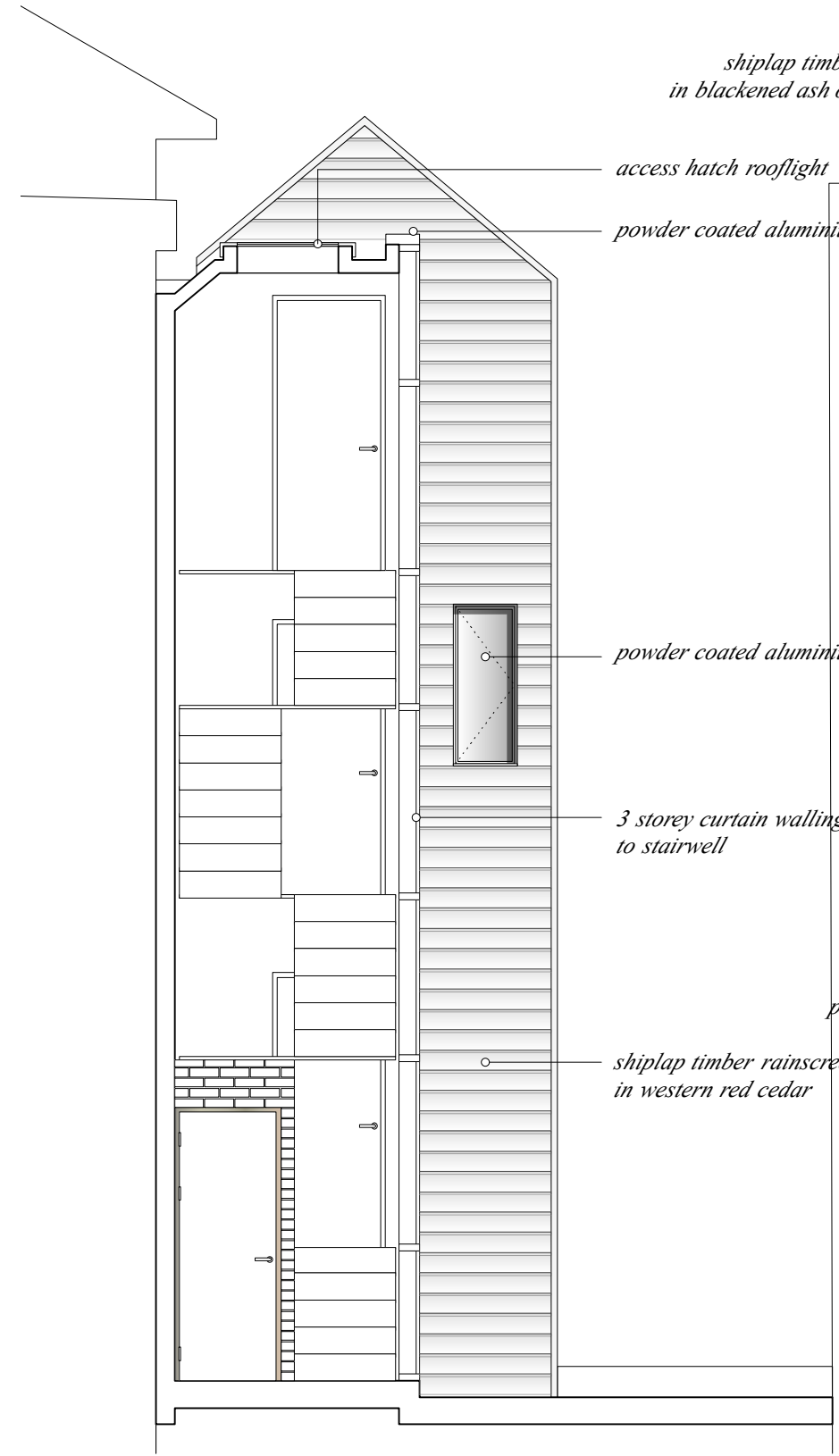
STAIR SECTION
