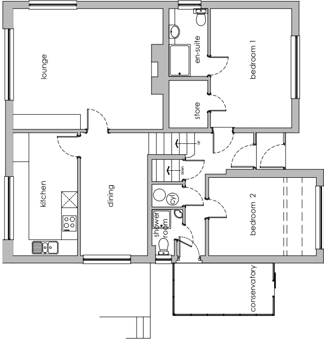
GROUND FLOOR PLAN (SPRING TIDE)
