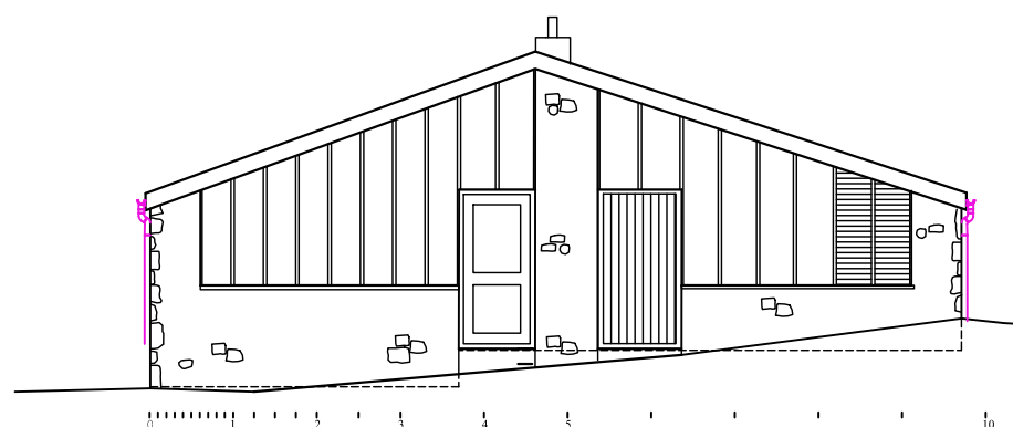
East Elevation
