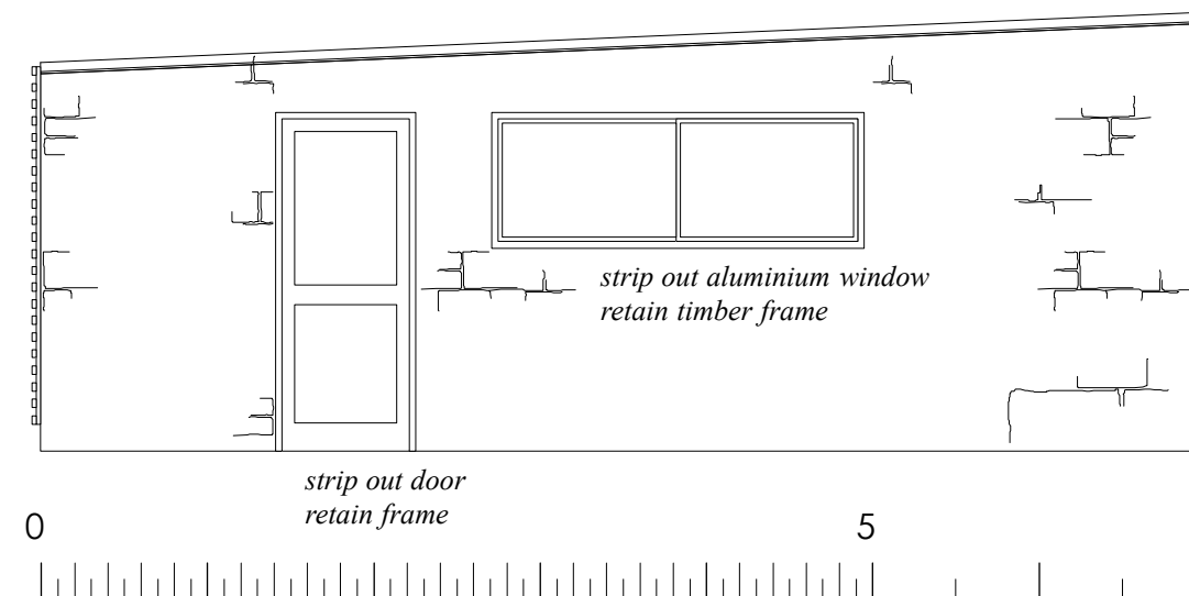
SIDE ELEVATION
