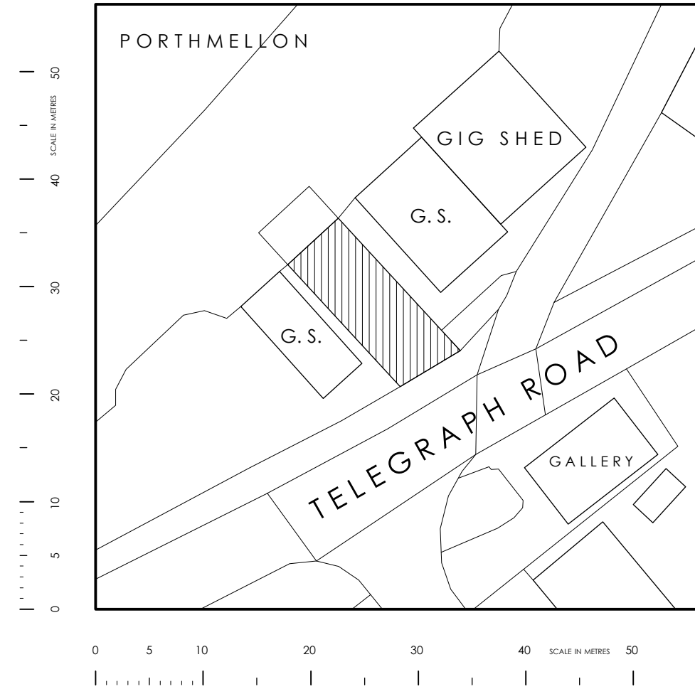
BLOCK PLAN - 1:500
