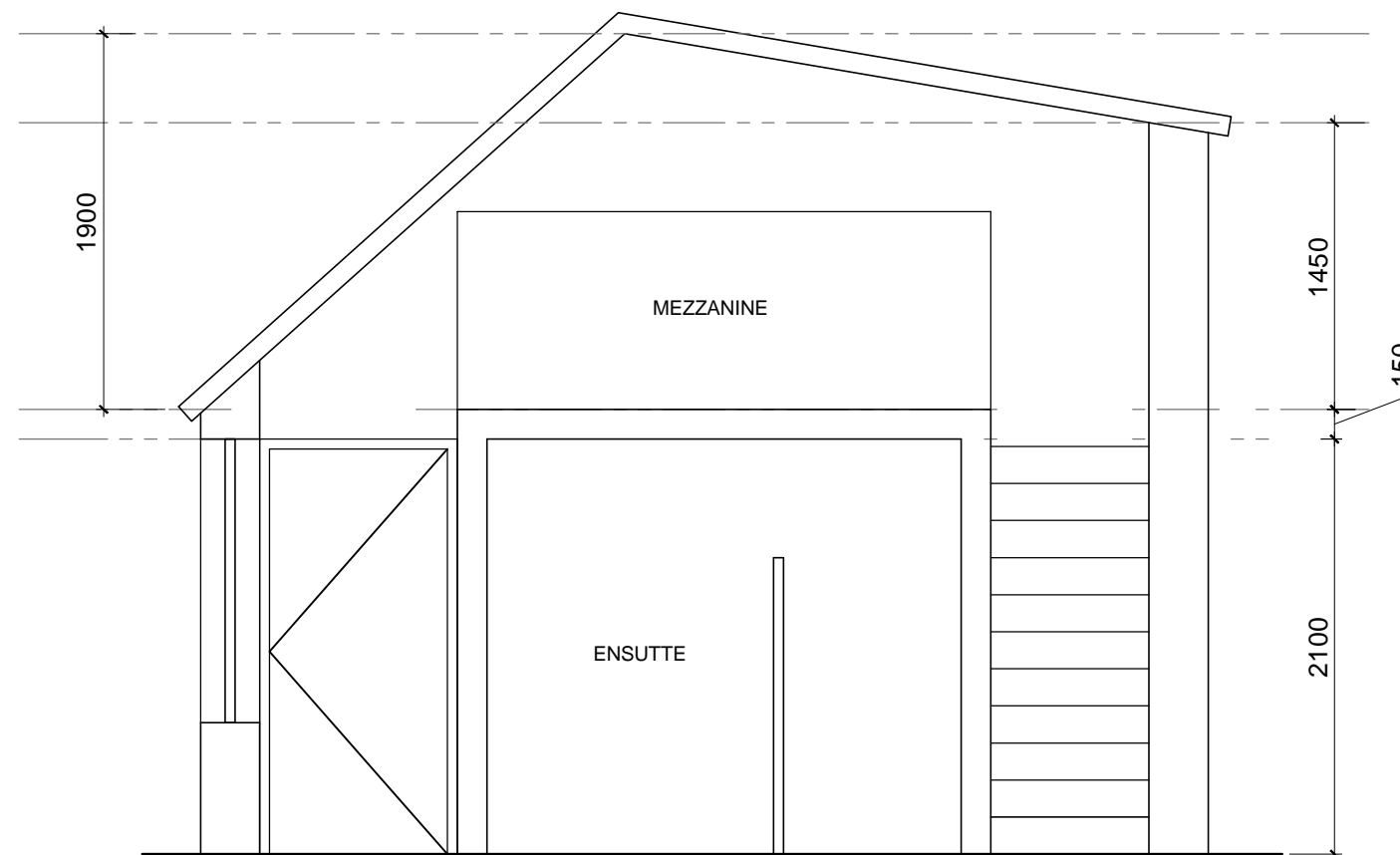
1 SECTION THRO MEZZANINE SCALE - 1:50
