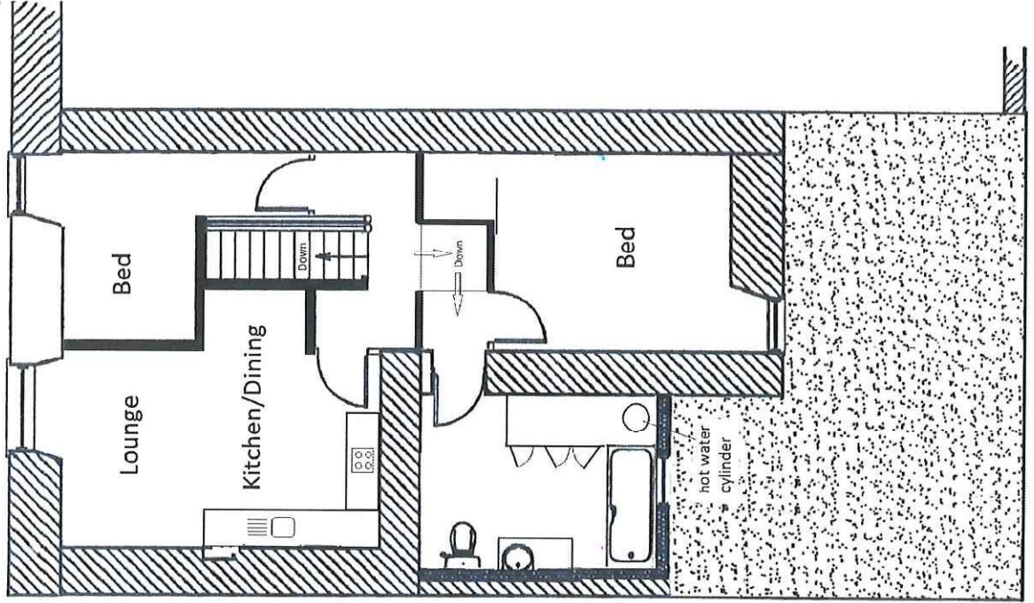
First Floor
