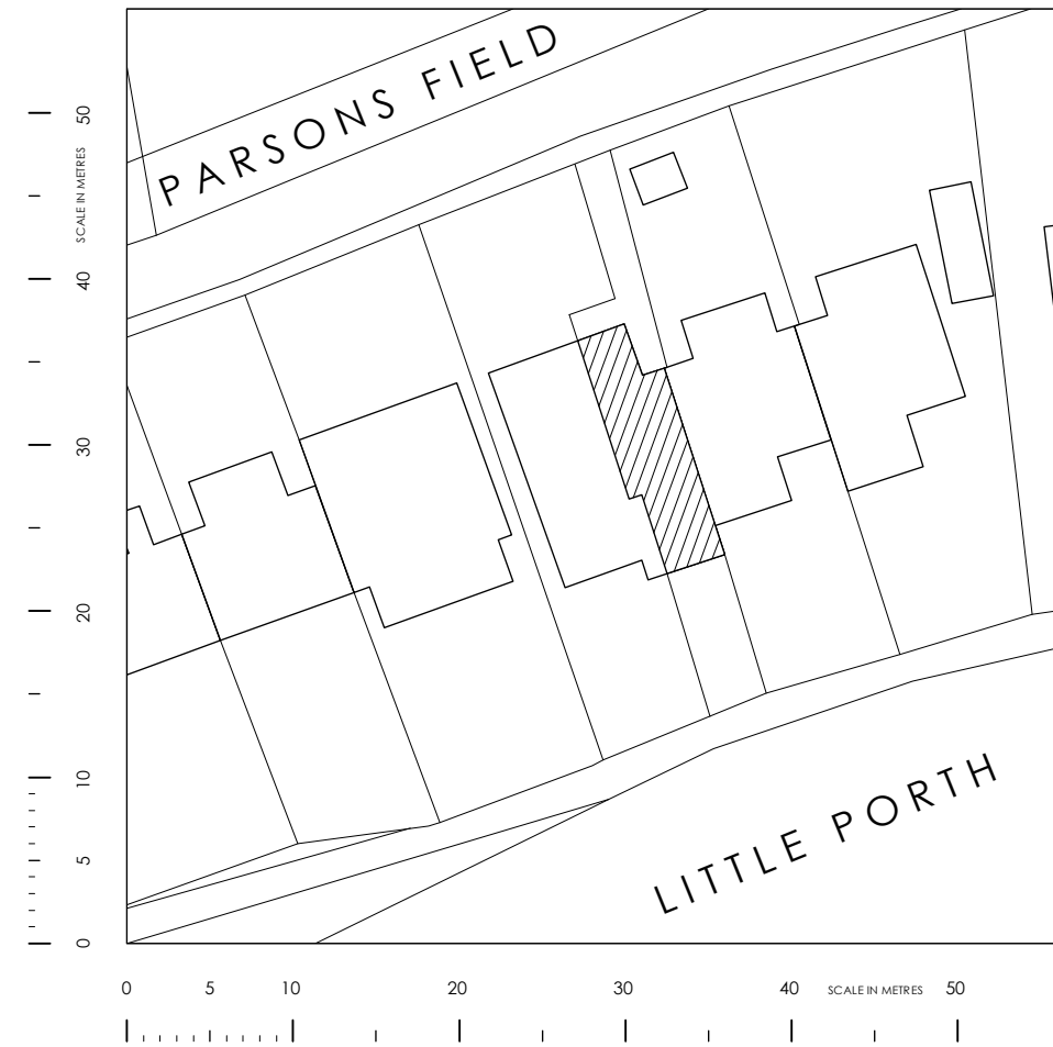
BLOCK PLAN - 1:500
