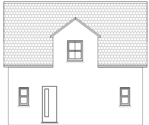
Front Elevation North-East
