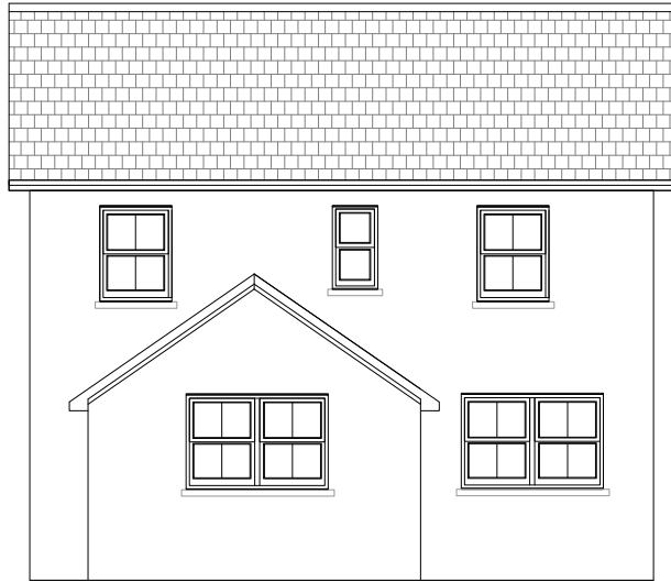
Rear Elevation West-South
