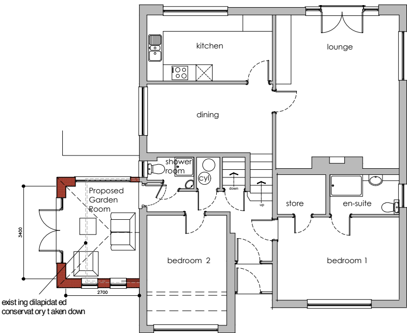
GROUND FLOOR PLAN (SPRING TIDE)
