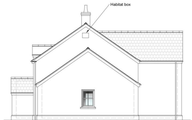
North Elevation
