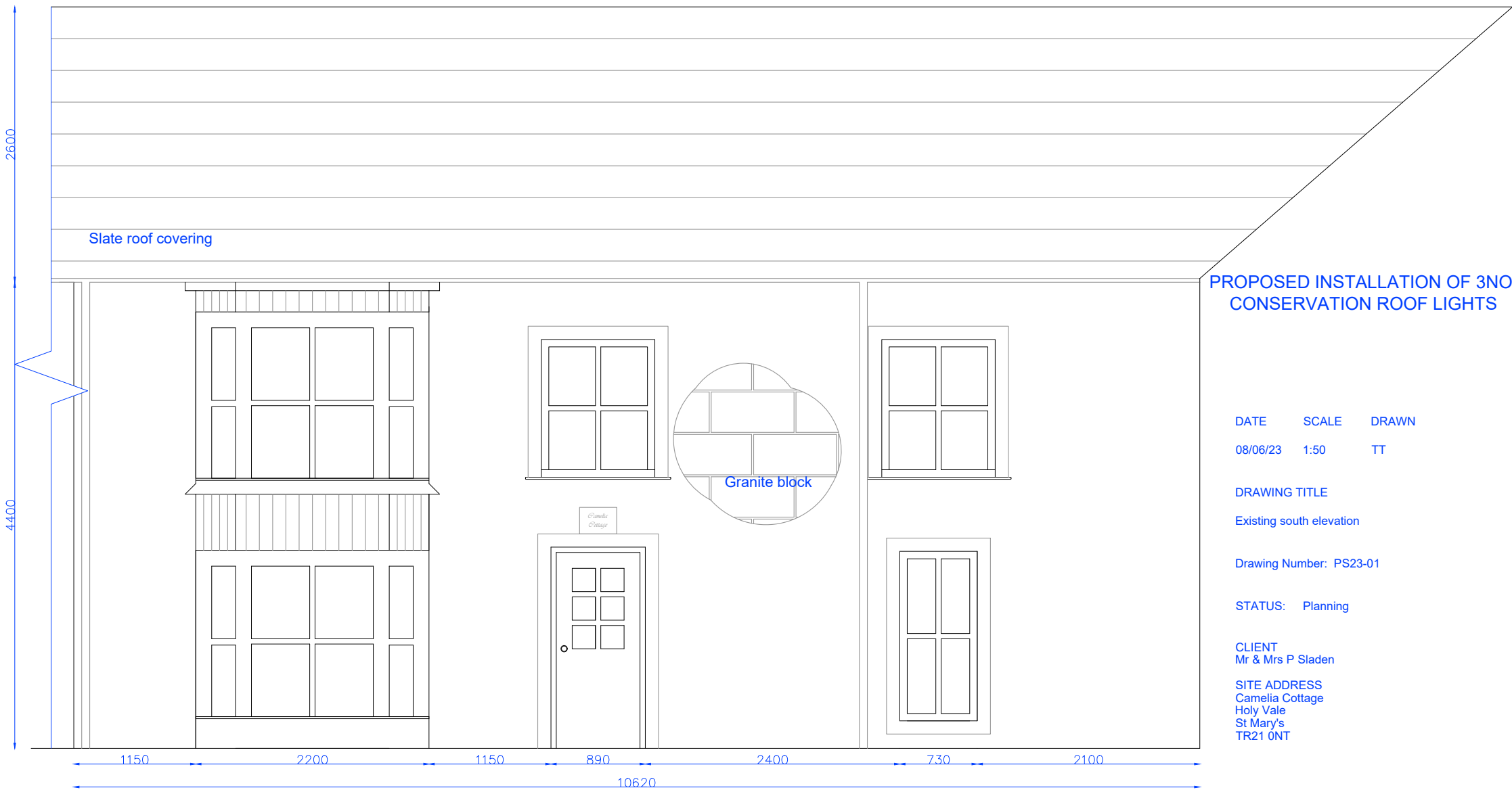
Front elevation as existing
