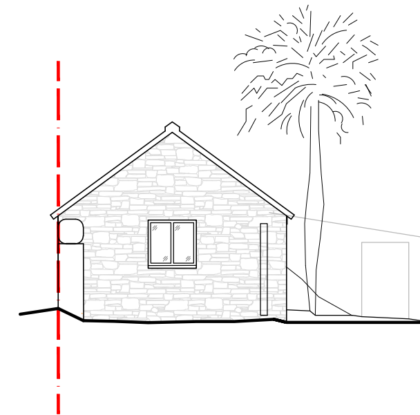
Existing South East Elevation
