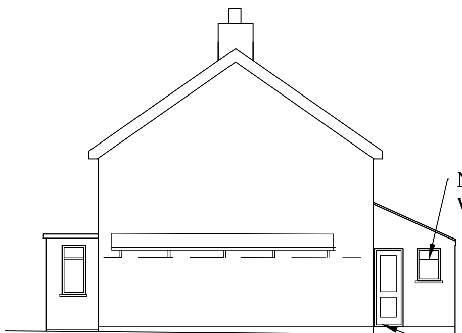
SOUTH ELEVATION
