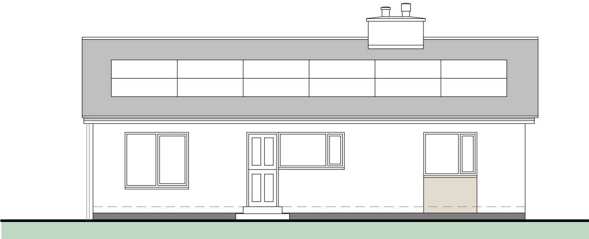
West Elevation
